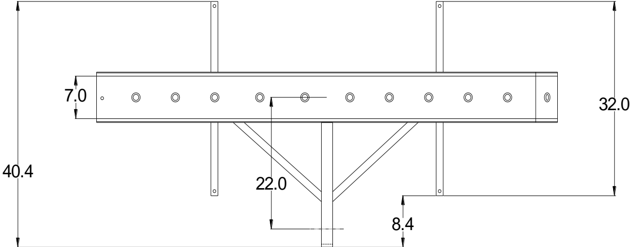
TOP VIEW
