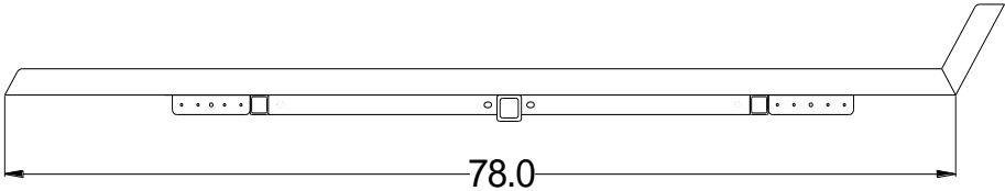
END VIEW
